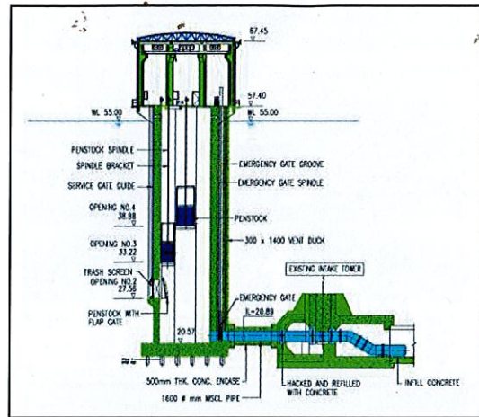
Cross Sectional View of Draw-off Tower No.1
