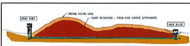
Cross Sectional View of Draw-off Tunnel
